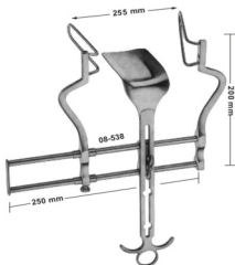
08-538 BALFOUR Lateral blades 105 mm deep Center blade 107 x 59 mm
