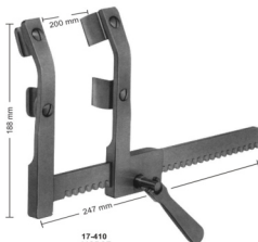
17-410 MORSE Sternotomy spreader for adults, with moveable double, each blade 19x19 mm
