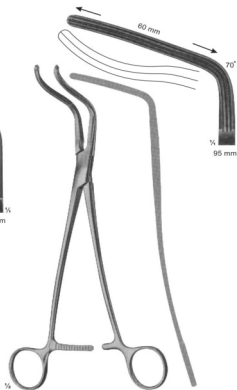
17-270 DE BAKAY 265 mm
