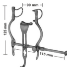
08-534 BALFOUR-BABY Lateral blades 27 mm deep Center blade 21x24 mm
