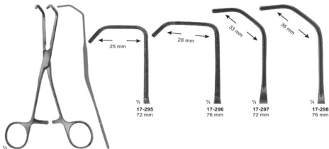
17-295 - 298 COOLEY 165 mm, 165 mm 175 mm, 180 mm
